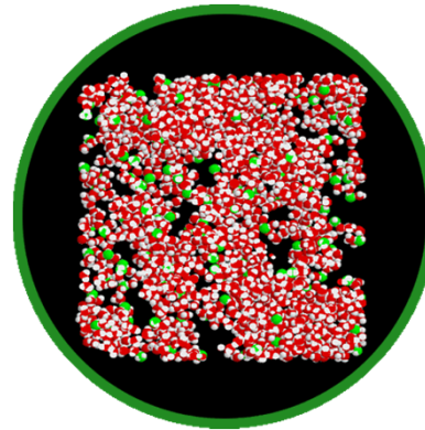
membrane morphology
