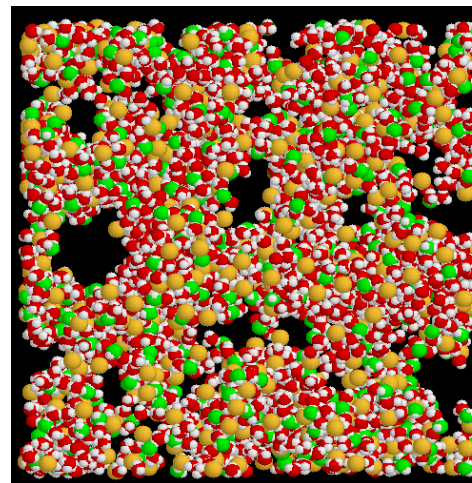
membrane morphology
