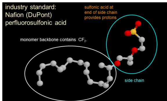
polymer chemistry
